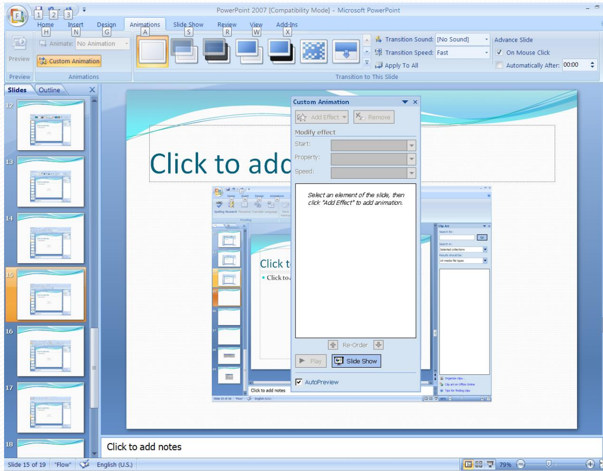
Slika 6. Custom Animation
